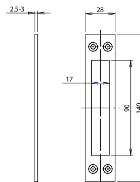
FRAME STRIKE PLATE
